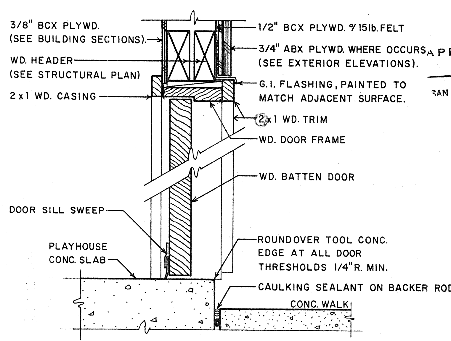
3 TYPICAL DOOR DETAIL 3" = 1'-0"
