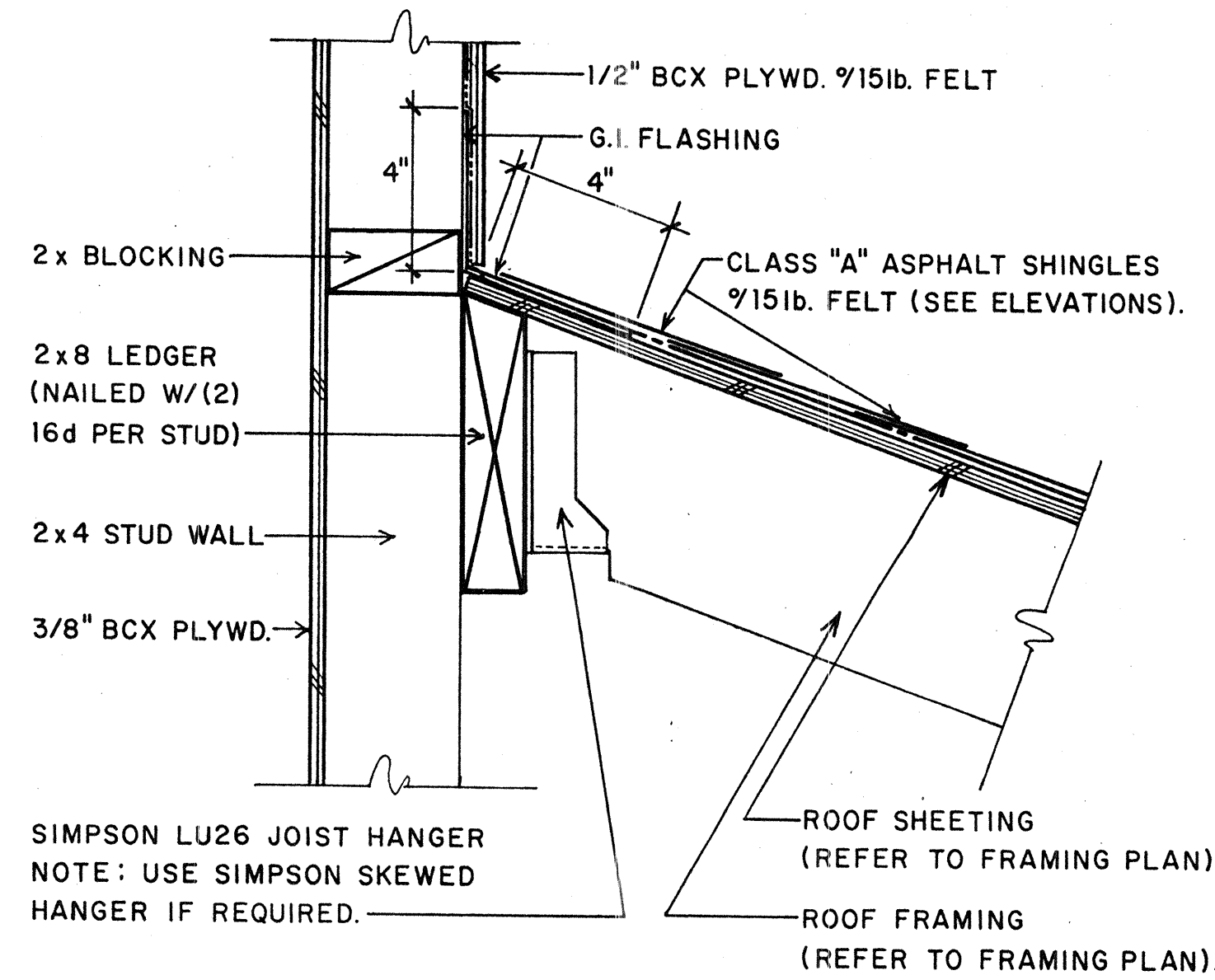
4 WALL TO ROOF DETAIL 3" = 1'-0"
