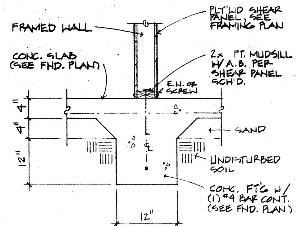
10 FTG DETAIL 1" = 1'-0"
