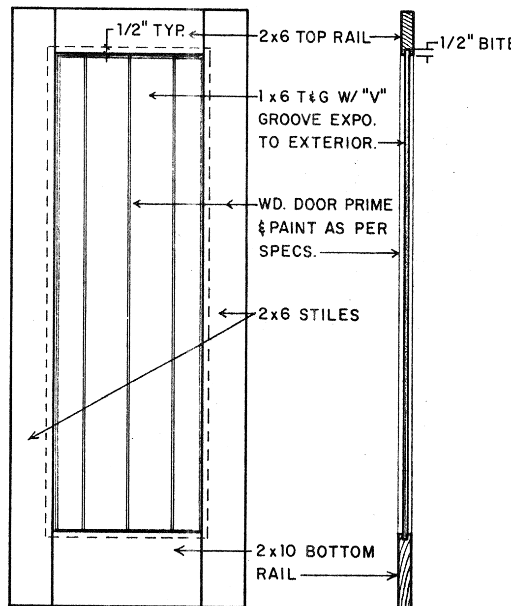
6 TYPICAL BATTEN DOOR DETAIL 1" = 1'-0"
