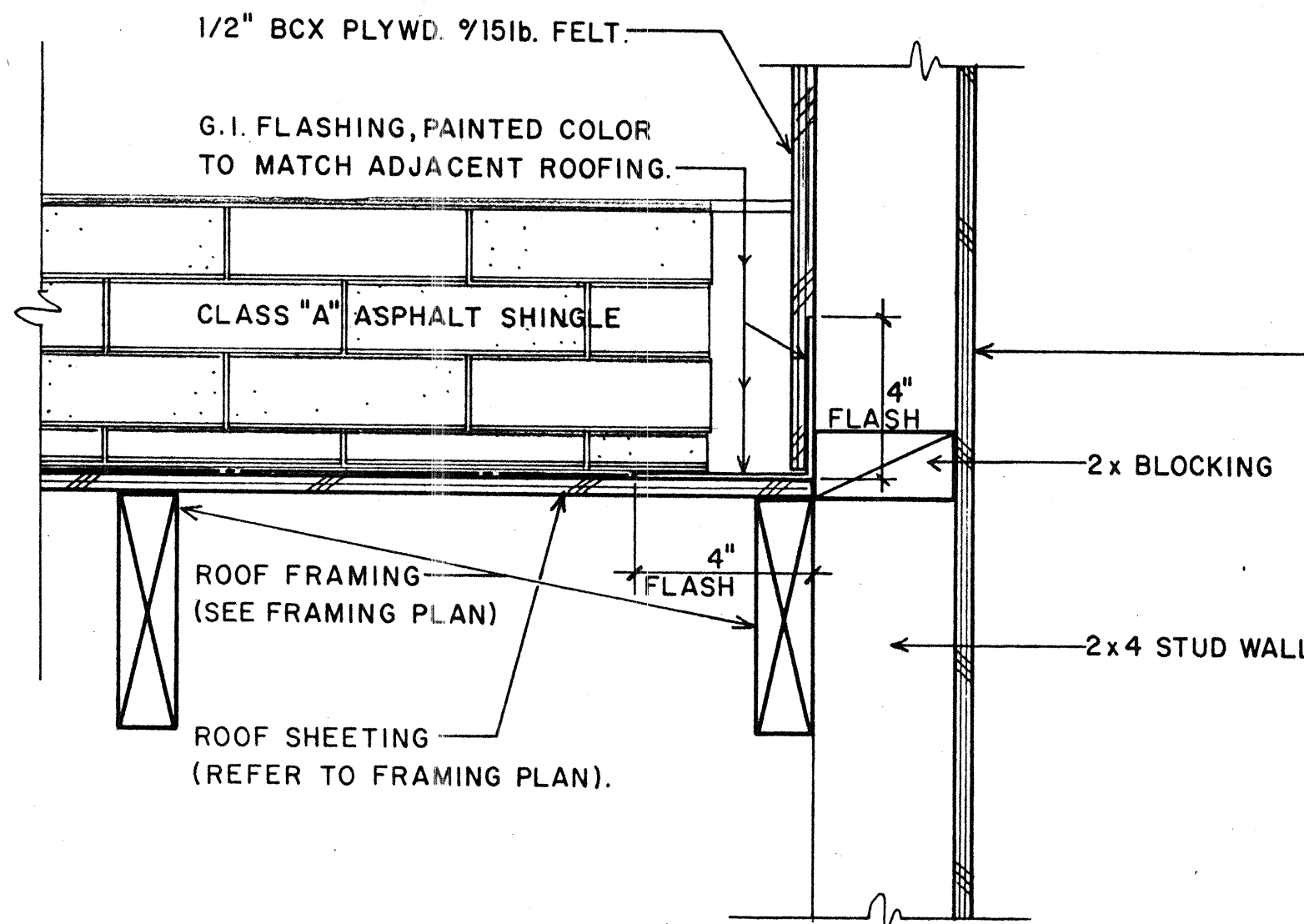
5 WALL TO ROOF RAKE DETAIL 3" = 1'-0"
