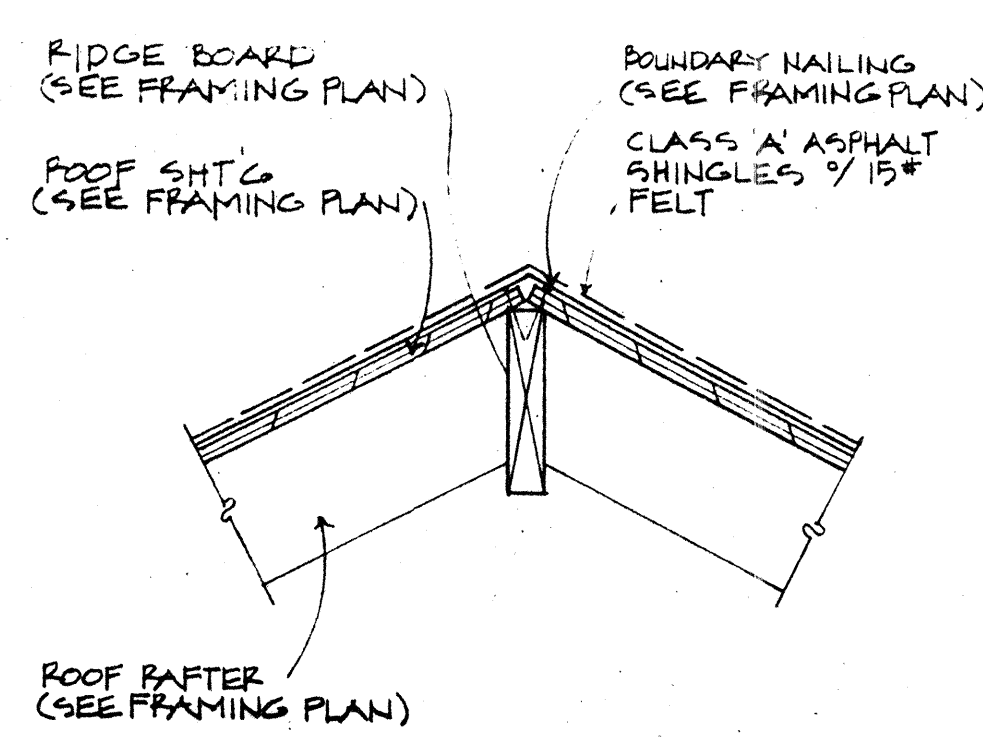
7 RIDGE DETAIL 1/2" = 1'-0"
