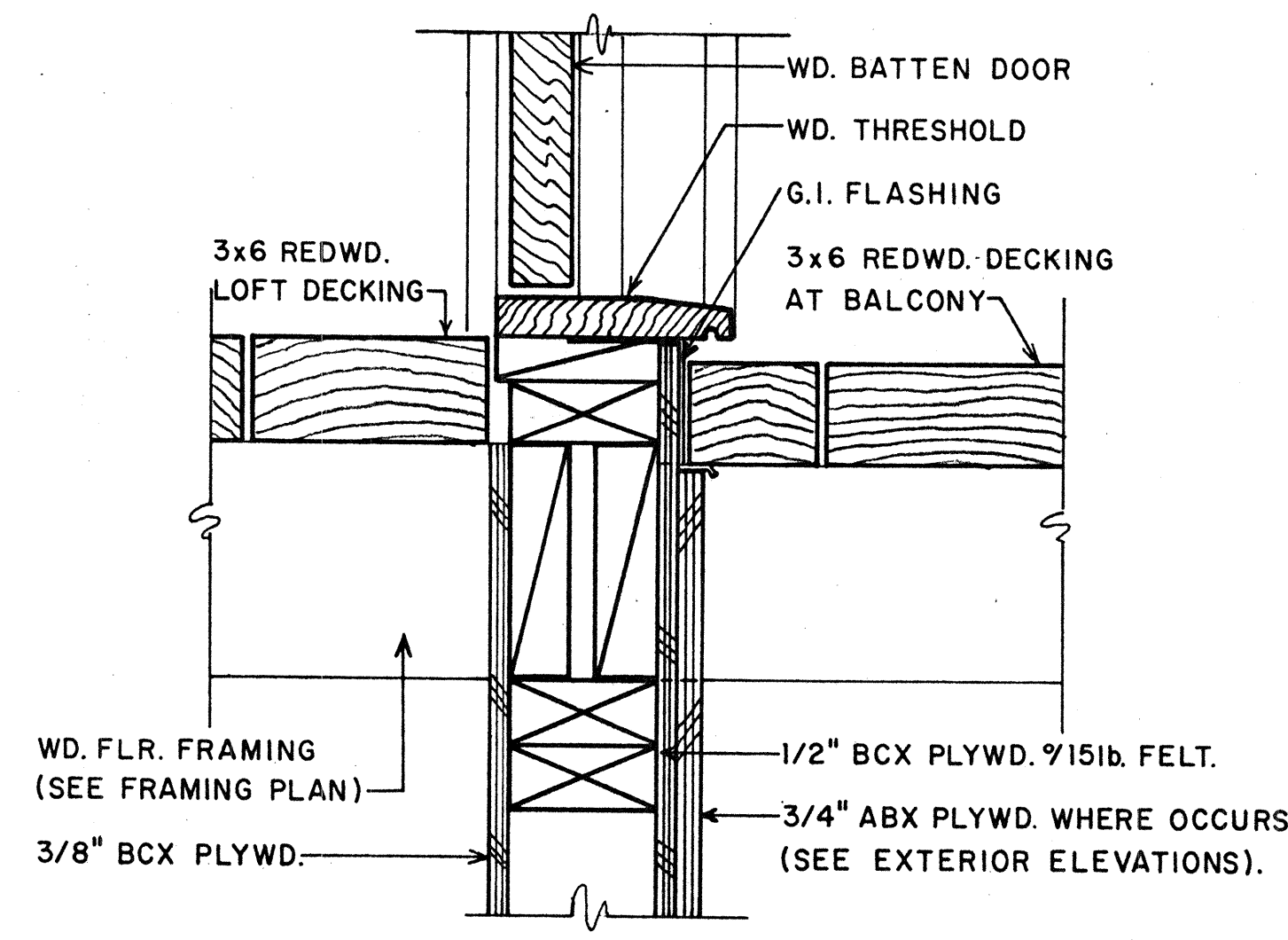
1 LOFT DOOR THRESHOLD DETAIL 3" = 1'-0"
