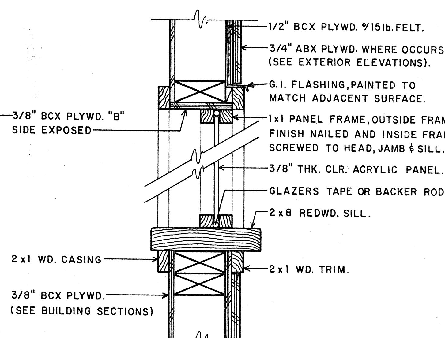
2 TYPICAL WINDOW DETAIL 3" = 1'-0"
