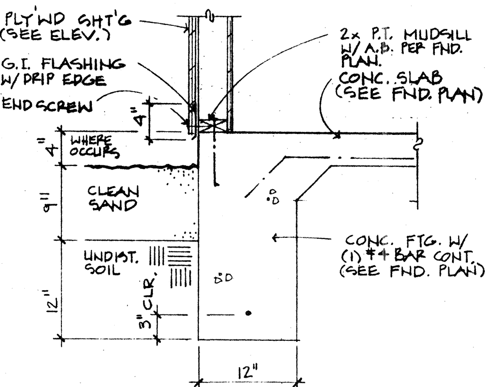
9 FTG DETAIL 1" = 1'-0"
